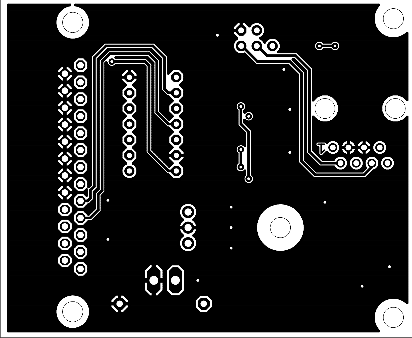
mm 25 x mm 25 Abmessungen (c) www.digital-brain.de - Sven Brandt
